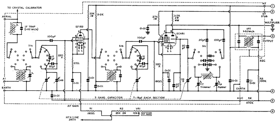
The front-end of the receiver (Electroniques type QP166). The bandswitch is shown in the 160 metre position. Only the coils and trimmers for 10 metres are shown; the others occupy corresponding positions on the other bandswitch contacts. The oscillator switch section SIC is fitted with shorting contacts.
